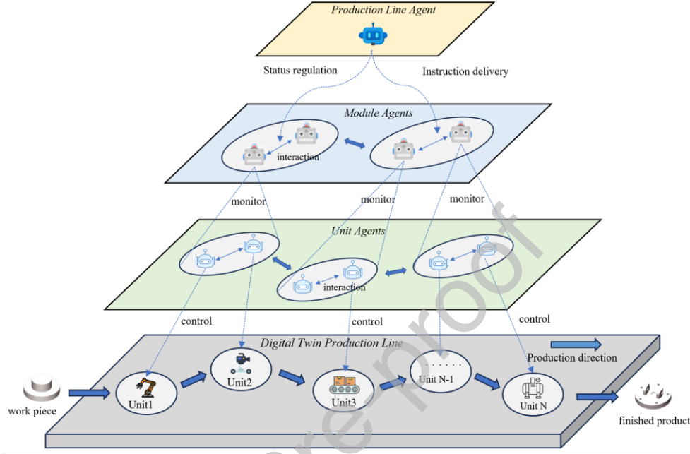
Fig. 7. Agent cooperative decision-making structure
