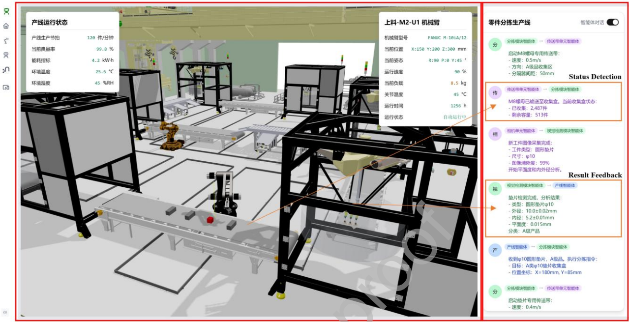
Fig. 16. Dynamic construction of the 3D production line model
