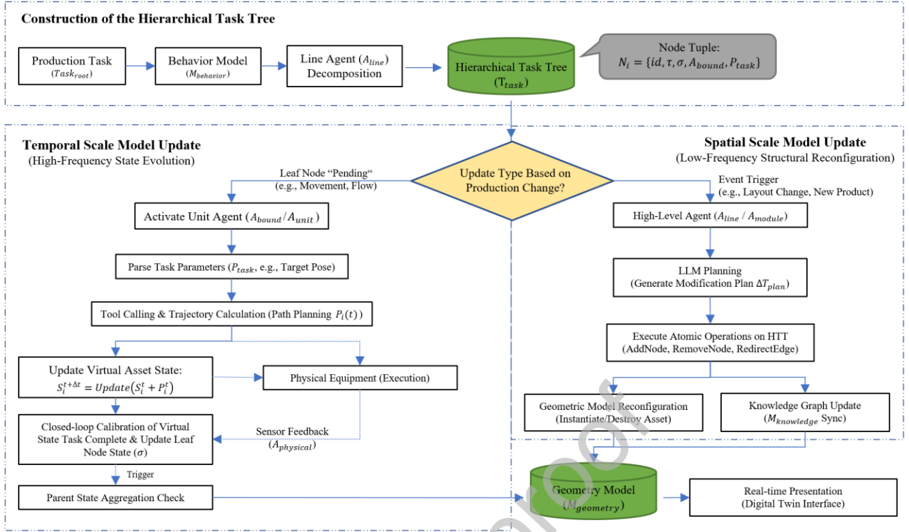
Fig. 10. Framework for HTT-driven multi-scale simulation.
